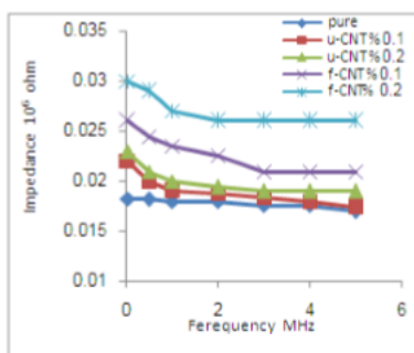
Fig(3) Variation of impedance as a function of frequency for different loading of CNTs
