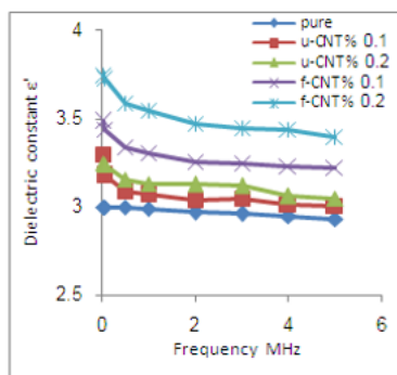
Fig(1) Variation of dielectric constant as a function of frequency for different loading of CNTs
