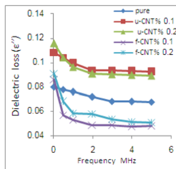
Fig(2) Variation of dielectric loss as a function of frequency for different loading of CNTs
